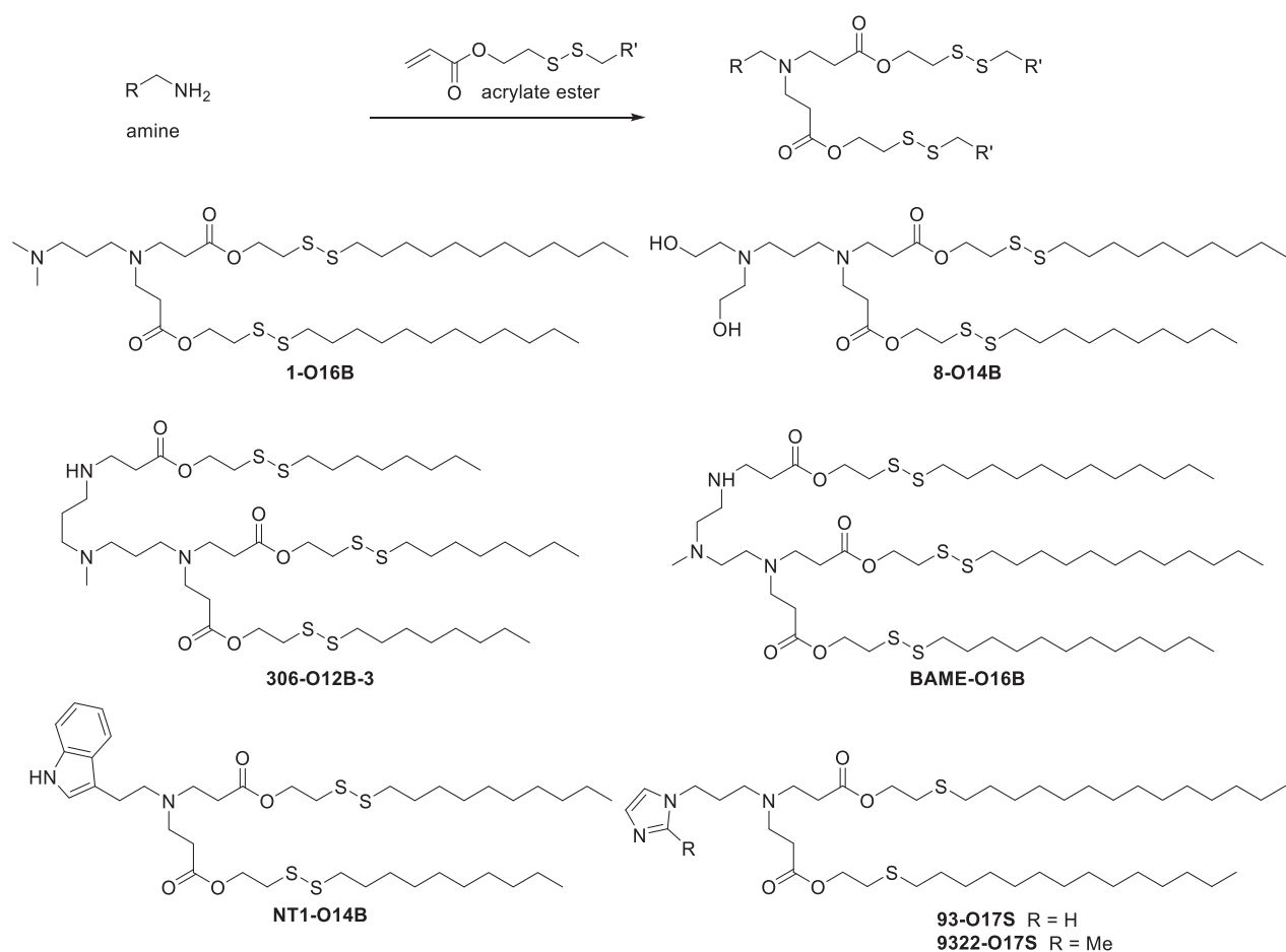
Figure 57. Chemical synthesis of bioreducible lipids.
