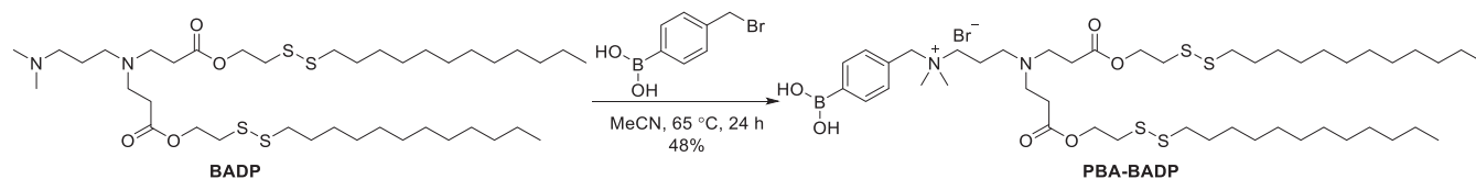
Figure 13. Chemical structure of PBA-BADP.
