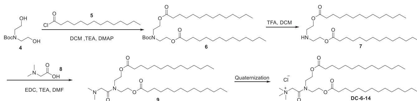
Figure 6. Chemical structure and synthetic route of DC-6-14.
