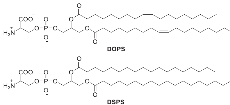
Figure 82. Chemical structures of representative phosphatidylserine.
