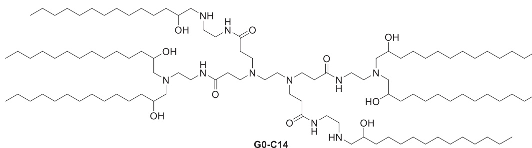
Figure 59. Synthesis of lipids from ring-opening reaction between amines and epoxides.
