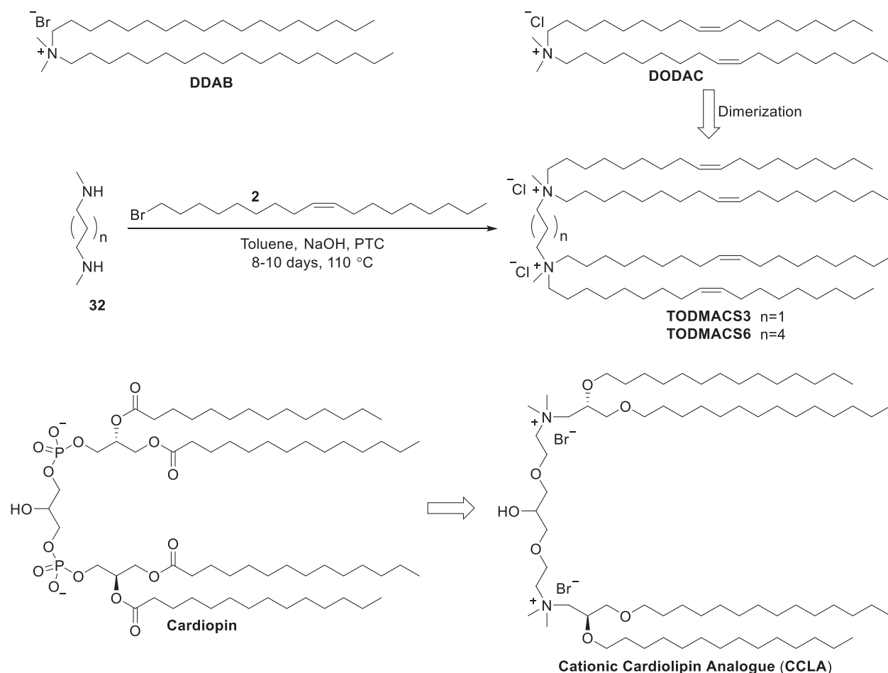
Figure 9. Synthesis of gemini diquatary ammoniums TODMACS3, TODMACS 6, and CCLA.
