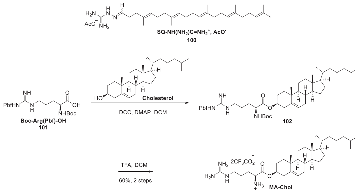
Figure 19. Chemical structures of squalene and cholesterol-derived guanidinium lipids.
